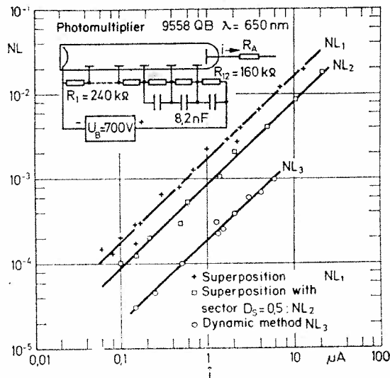
FIGURE 12. Jung's measurements of the nonlinearity of an EMI 9558 photomultiplier using 3 methods. (Courtesy, Z. Angew. Physik.)
