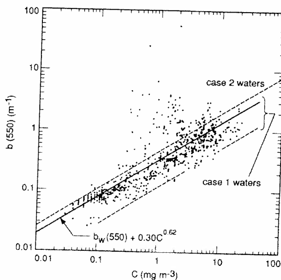
FIGURE 15 Measured scattering coefficients at \lambda = 550 \text{ nm} , b(550) , as a function of chlorophyll concentration C . Case 1 waters lie between the dashed lines. Case 2 waters lie above the upper dashed line, which is defined by b(550) = 0.45C^{0.62} . The solid line is the model of Eq. (6). (Redrawn from Gordon and Morel, 66 with permission.)
