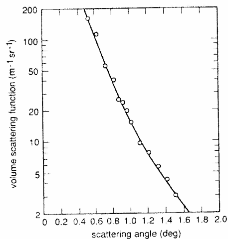
FIGURE 11 Detail of the forward scattering values of the "lake" volume scattering function seen in the top curve of Fig. 10. (Redrawn from Preisendorfer. 7 )
