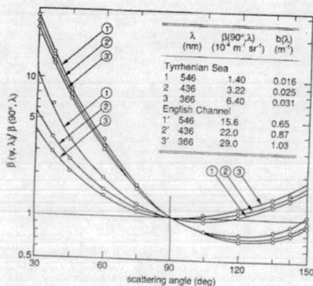
FIGURE 13 Wavelength dependence of total volume scattering functions measured in very clear (Tyrrhenian Sea) and in turbid (English Channel) waters. (Redrawn from Morel. 64 )
