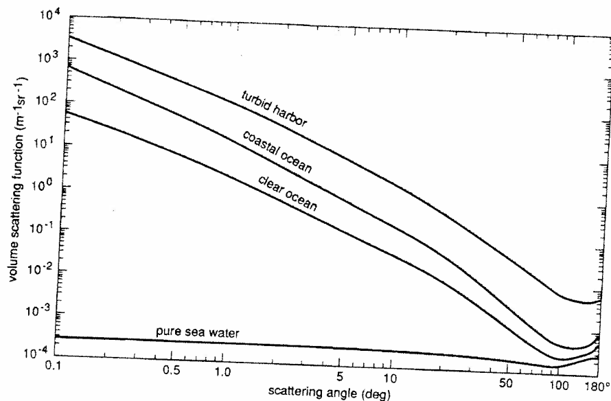
FIGURE 12 Measured volume scattering functions from three different natural waters and the computed volume scattering function for pure sea water, all at \lambda = 514 nm. (Redrawn from Petzold. 53 )
