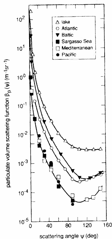
FIGURE 10 Particulate volume scattering functions \beta_p(\psi, \lambda) determined from in situ measurements in various waters; wavelengths vary. (Redrawn from Kullenberg, 59 with permission.)
