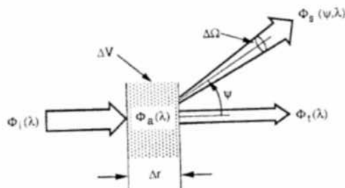
FIGURE 2 Geometry used to define inherent optical properties.
