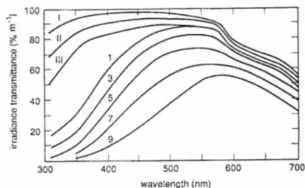
FIGURE 19 Percentage transmittance per meter of water of downwelling irradiance E_d as a function of wavelength for selected Jerlov water types. (Reproduced from Jerlov, 29 with permission.)
