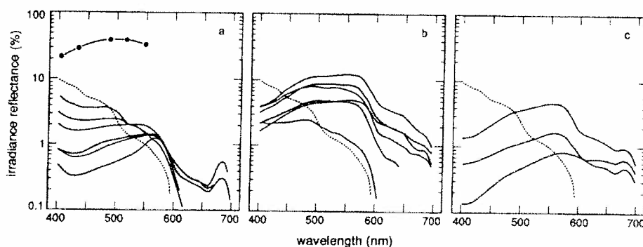
FIGURE 21 Measured spectral irradiance reflectances R(\lambda) from various waters. Panel (a) is from case waters with different quantities of phytoplankton; the dotted line is R(\lambda) for pure sea water. The heavy dots give values measured within a coccolithophore bloom. 20 Panel (b) is from case 2 waters dominated by suspended sediments and panel (c) is from case 2 waters dominated by yellow matter. (Redrawn from Sathyendranath and Morel, 79 with permission.)
